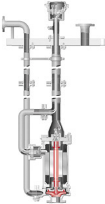
submersible pump with canned motor
